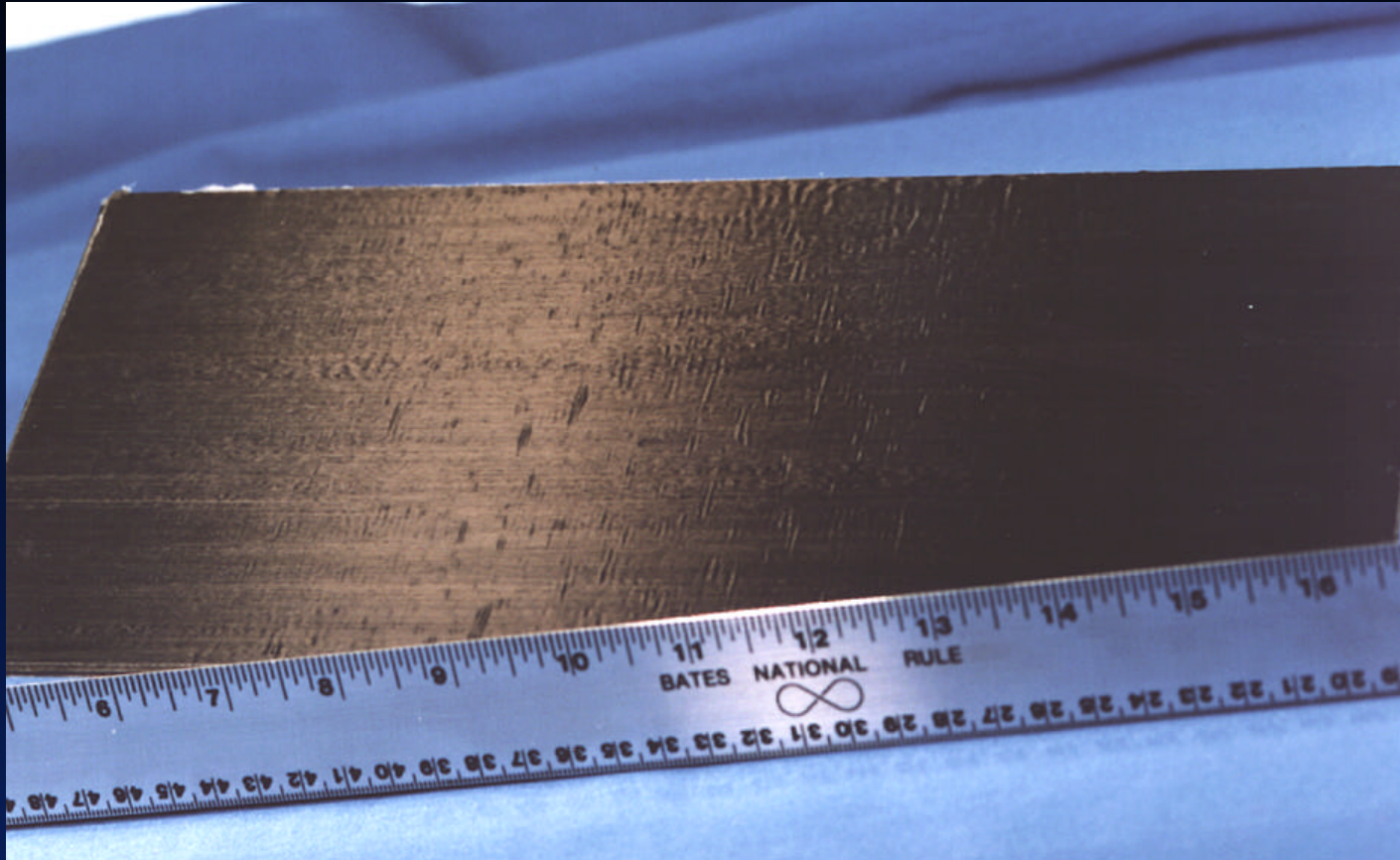
Fiber Waviness in a Carbon Fiber-Reinforced Thermoplastic Laminate (Amoco T300/P1700, 6 x 12cm, 12 plies)
