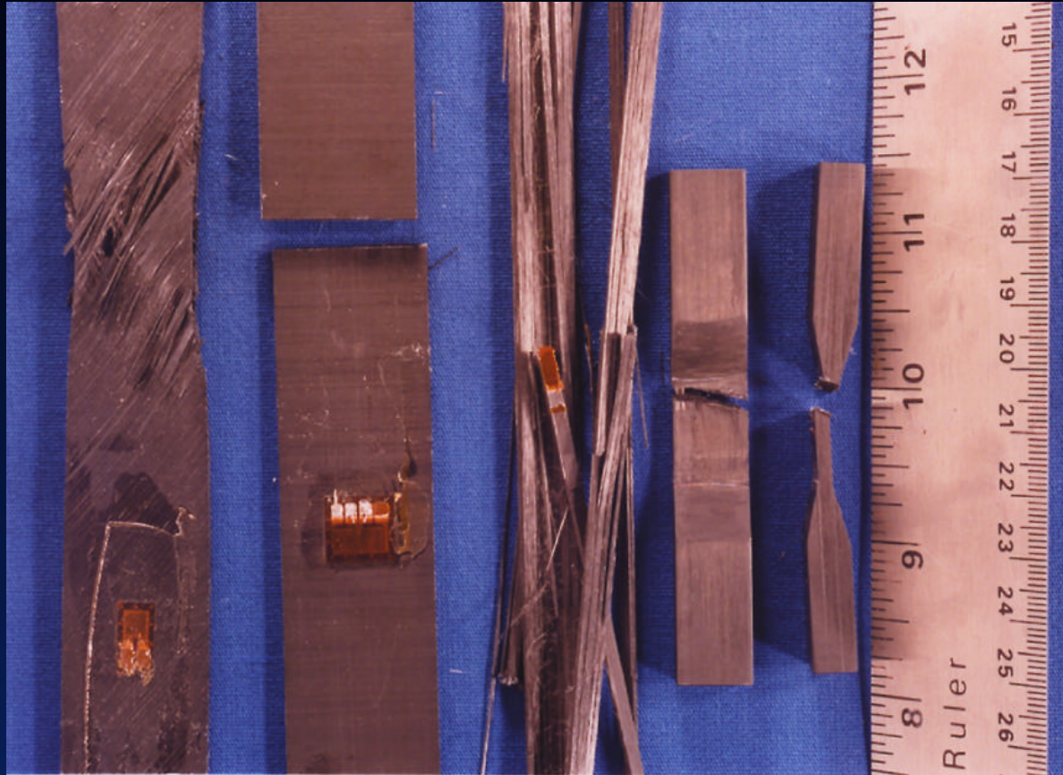
Tension & Compression Failures in Carbon Fiber-Reinforced Thermoplastic Laminates (Amoco T300/P1700)
