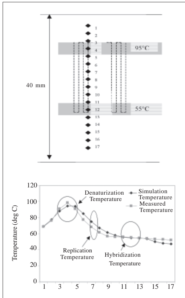
Figure 9 (a) Measuring points along the bottom glass surface, (b) measured and simulated temperature distributions on the glass surface of the PCR chip
