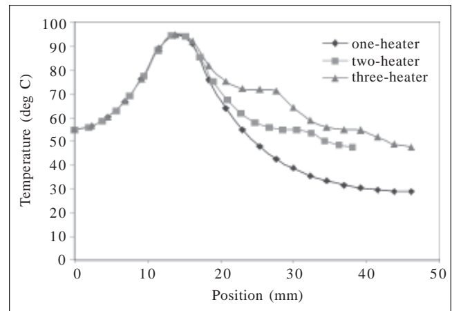
Figure 2 Comparison of Temperature Distribution Along the PCR Chip for Three Different Heater Designs
