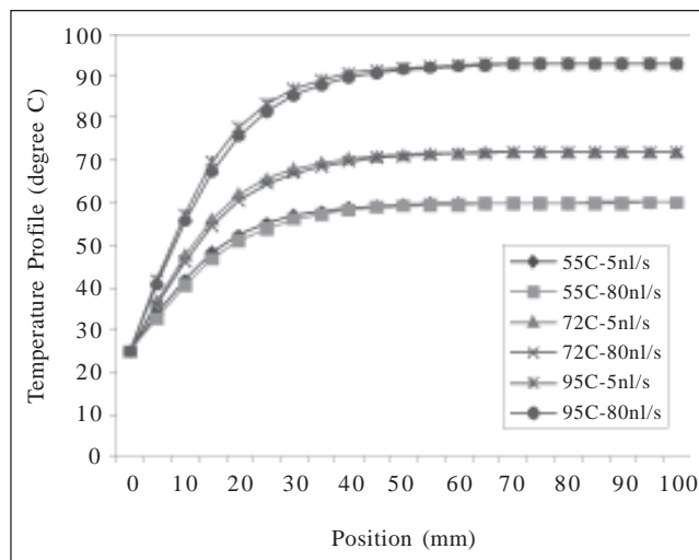
Figure 3 Simulation Results of the Thermal Entry Length for Different Temperatures and Flow Rates
