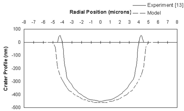
Fig. 1 Single shot ablated crater, E_{\text{pulse}}=13.8 \mu\text{J}
